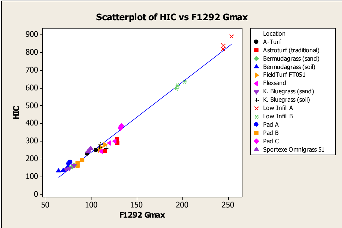
Figure 14. Scatterplot of the relationship between Gmax and HIC using the F1292 device with test locations identified
