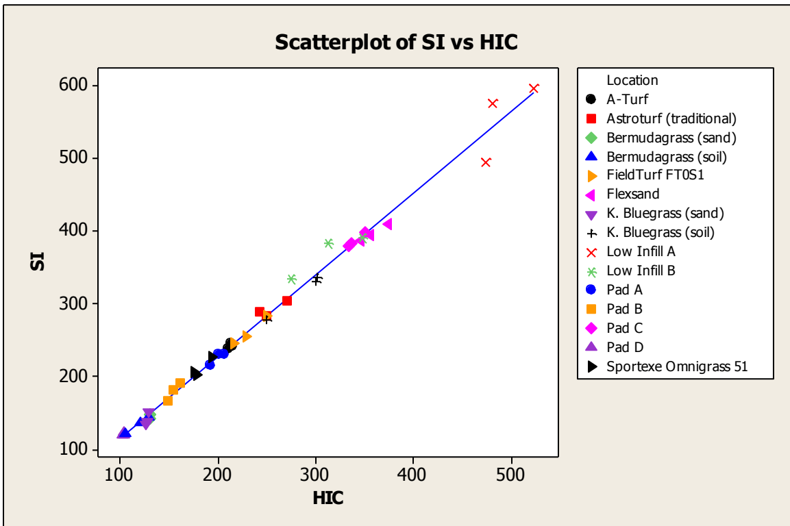
Figure 18. Scatterplot of the relationship between SI and HIC using the Clegg with test locations identified
