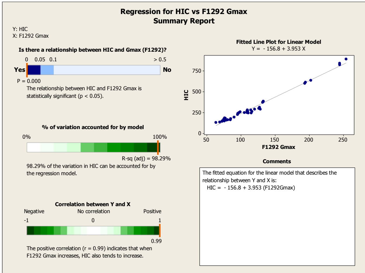
Figure 13. Summary of regression test for Gmax and HIC with the F1292 device
