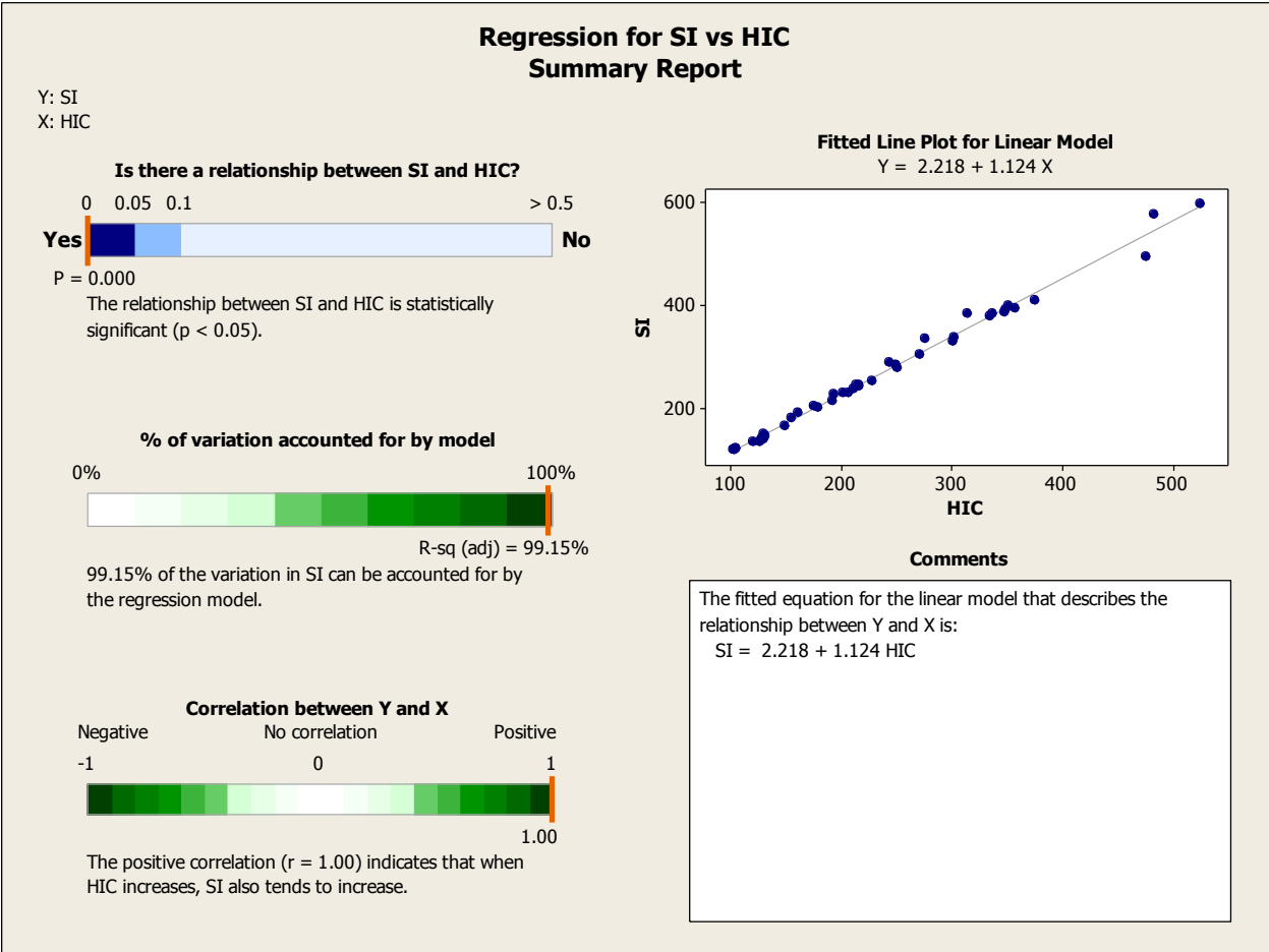
Figure 17. Summary of regression test for Gmax and HIC with the Clegg
