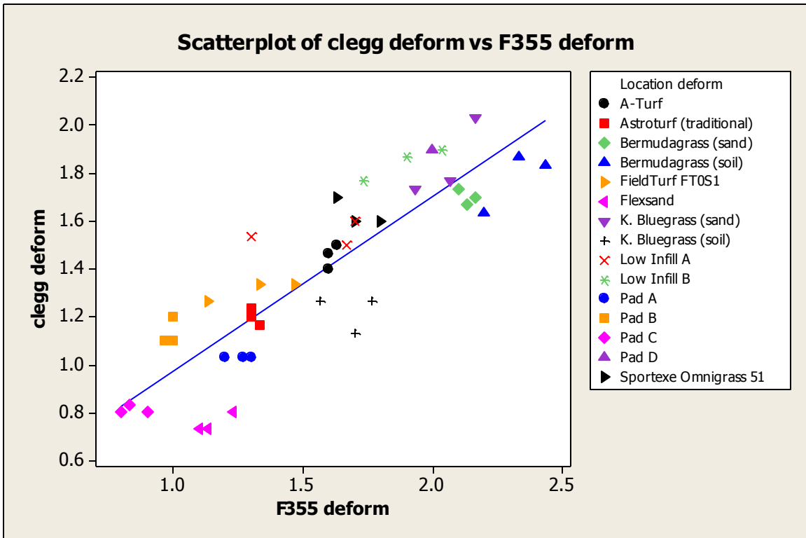
Figure 20. Scatterplot of the relationship between the F355 and Clegg for vertical deformation
