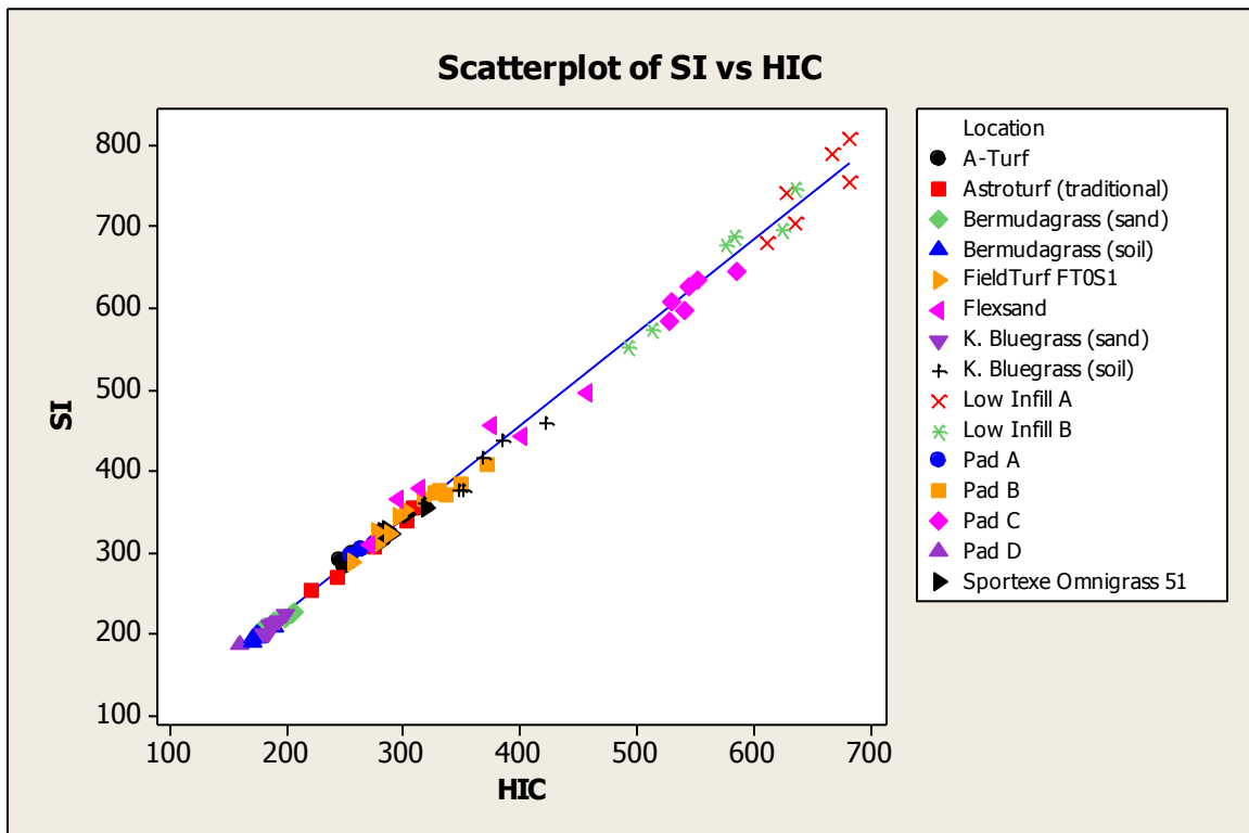
Figure 16. Scatterplot of the relationship between SI and HIC using the F355 device with test locations identified
