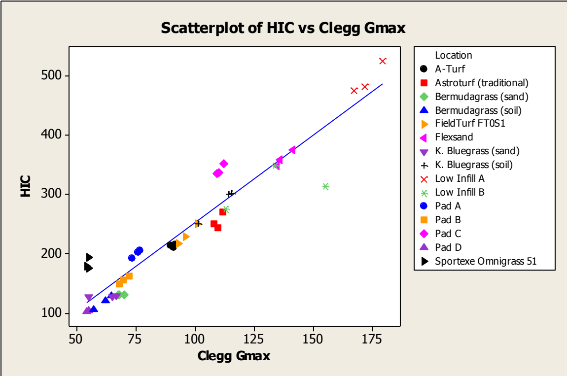
Figure 12. Scatterplot of the relationship between Gmax and HIC using the Clegg with test locations identified
