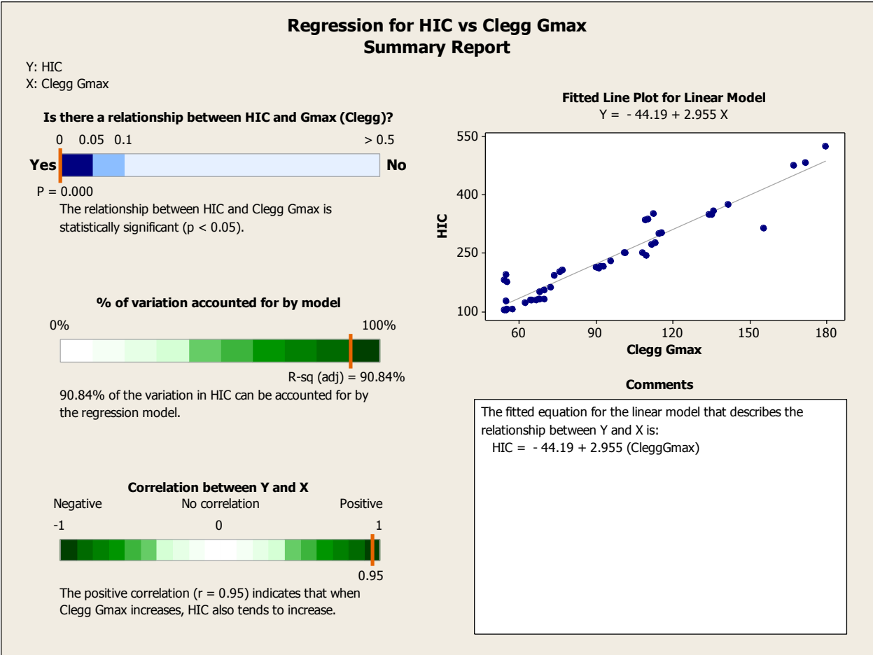
Figure 11. Summary of regression test for Gmax and HIC with the Clegg
