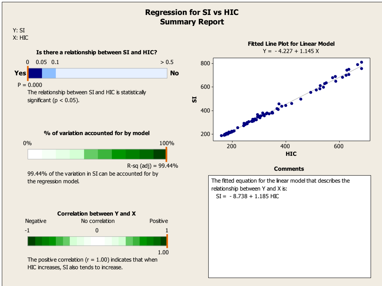
Figure 15. Summary of regression test for SI and HIC with the F355 device
