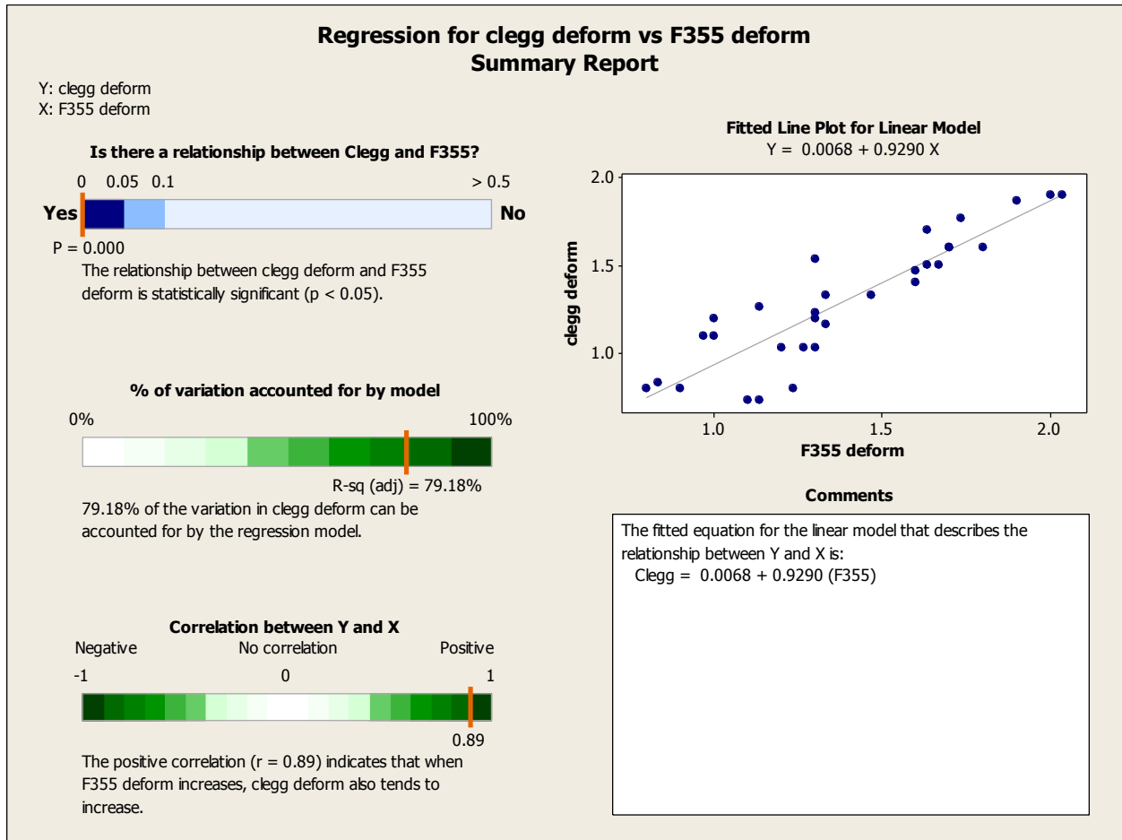
Figure 19. Summary of regression test for the F355 and Clegg for vertical deformation
