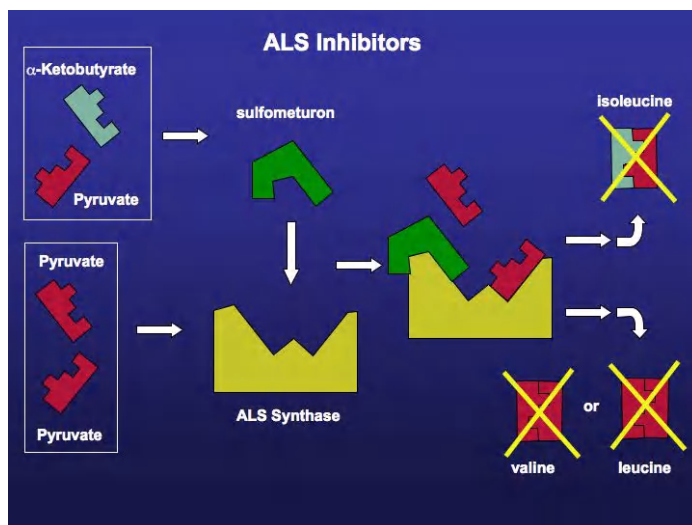
Figure 1. Illustration of the sulfometuron molecule binding with ALS Synthase and preventing the production of three amino acids – isoleucine, leucine, and valine.
